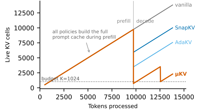
Figure 4: Live KV cells through prefill and decode on Llama-3.2-1B. Only \mu KV compacts to its budget and stays bounded.
