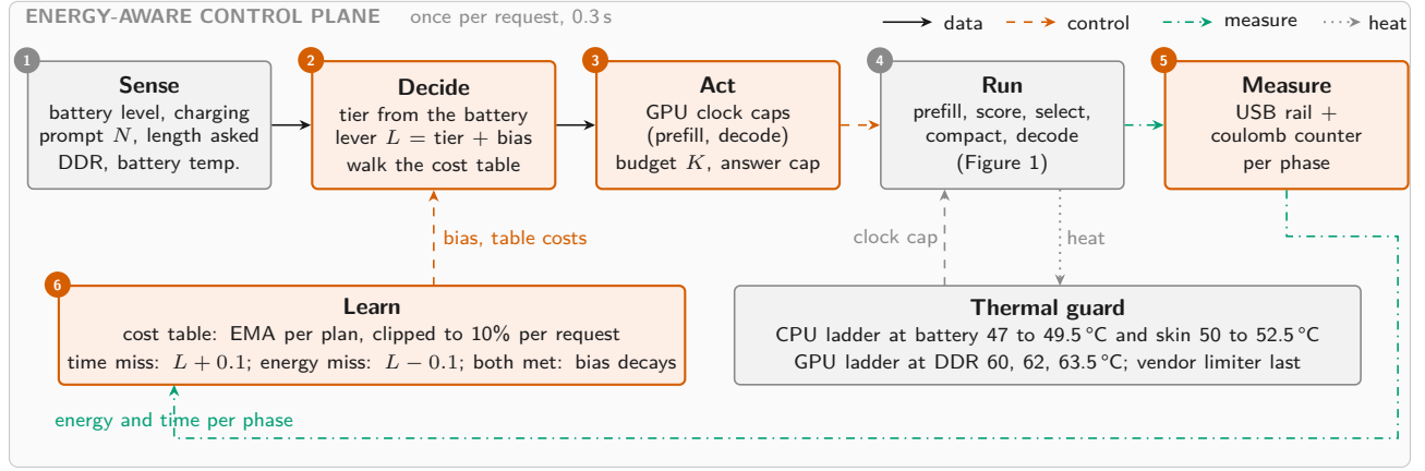
Figure 3: The energy-aware control plane, once per request: sense, decide, act, run, measure, learn. The thermal guard acts on the clock beside it.
