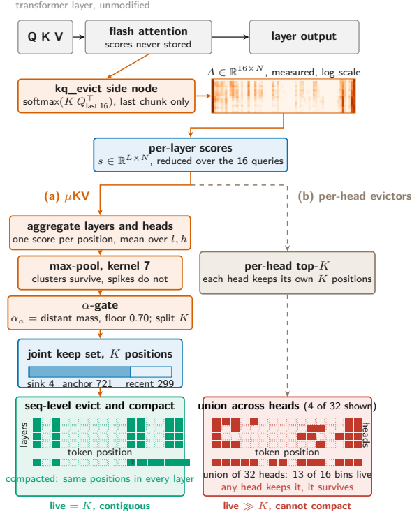
Figure 2: Scores, selection and the two outcomes. Heatmap and keep sets are measured on Llama-3.2-1B, layer 8, 16 position bins: the union over 32 heads keeps 13 bins, the joint set 6.
