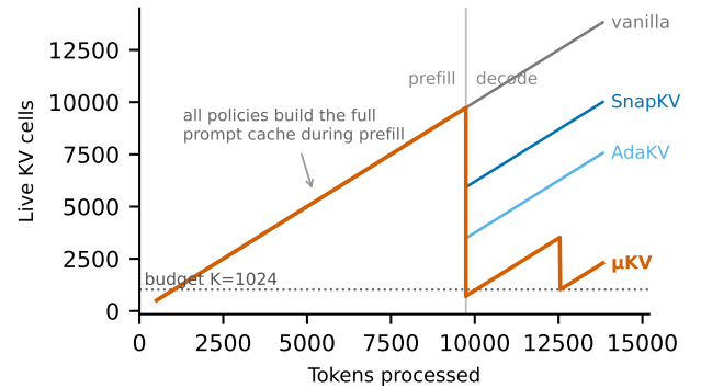
Figure 2: Live KV cells through prefill and decode, Llama-3.2-1B on the phone CPU. Every policy builds the full prompt cache. Neither per-head evictor returns to its budget; \mu KV compacts to 721 and holds near 2K.
