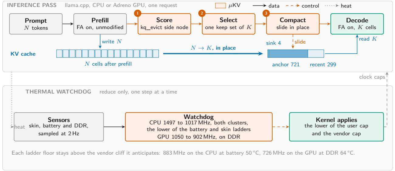
Figure 1: \mu KV on the phone. Top: the inference pass; scoring, selection and compaction (1 to 3) are the only changes. Bottom: the watchdog, which steps each clock cap down a ladder anchored above the vendor cliff.
