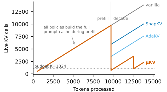
Figure 2: Live KV cells through prefill and decode on Llama-3.2-1B, phone CPU. Every policy builds the full prompt cache. Neither per-head evictor returns to its budget; \mu KV compacts to 723 cells and its re-eviction holds the cache near 2K.
