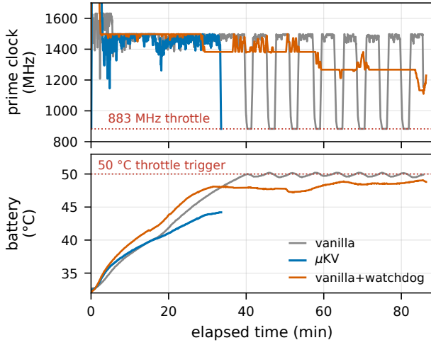
Figure 3: Bonsai-8B on the CPU from a cold start: prime clock and battery for the full cache, \mu KV, and the full cache with the watchdog (ablation).
