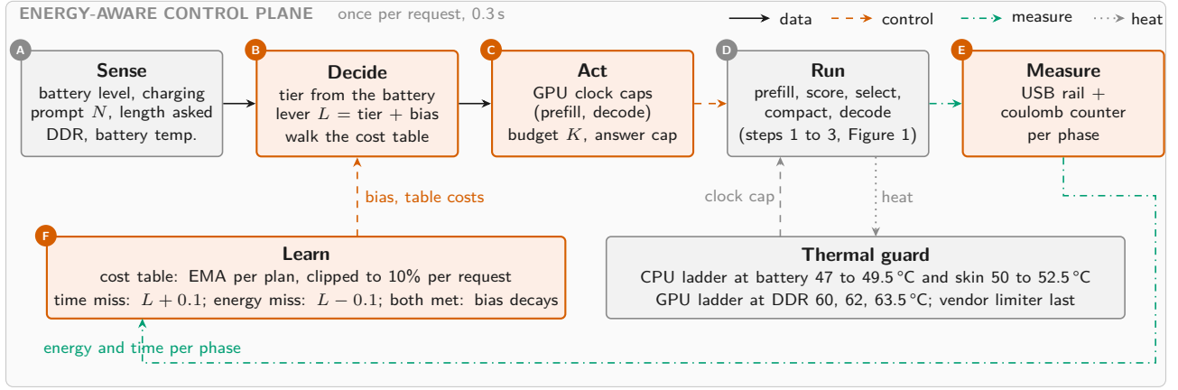
Figure 3: The energy-aware control plane, once per request, lettered A to F so the stages never collide with the numbered components of Figure 1. Stage D is that figures steps 1 to 3. The thermal guard acts on the clock beside it.
