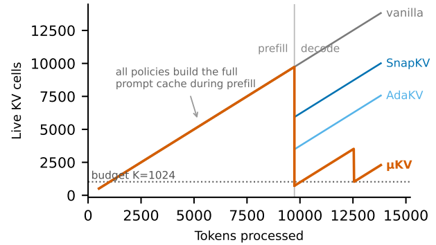
Figure 4: Live KV cells through prefill and decode on Llama-3.2-1B. Only μKV compacts to its budget and stays bounded.
