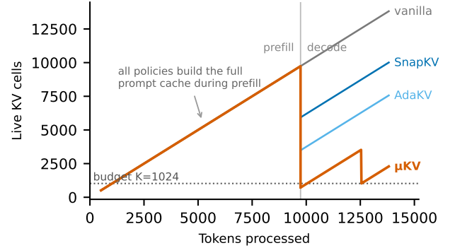
Figure 4: Live KV cells through prefill and decode on Llama-3.2-1B, phone CPU. Every policy builds the full prompt cache. Neither per-head evictor returns to its budget; μKV compacts to 723 cells and its re-eviction holds the cache near 2K.
