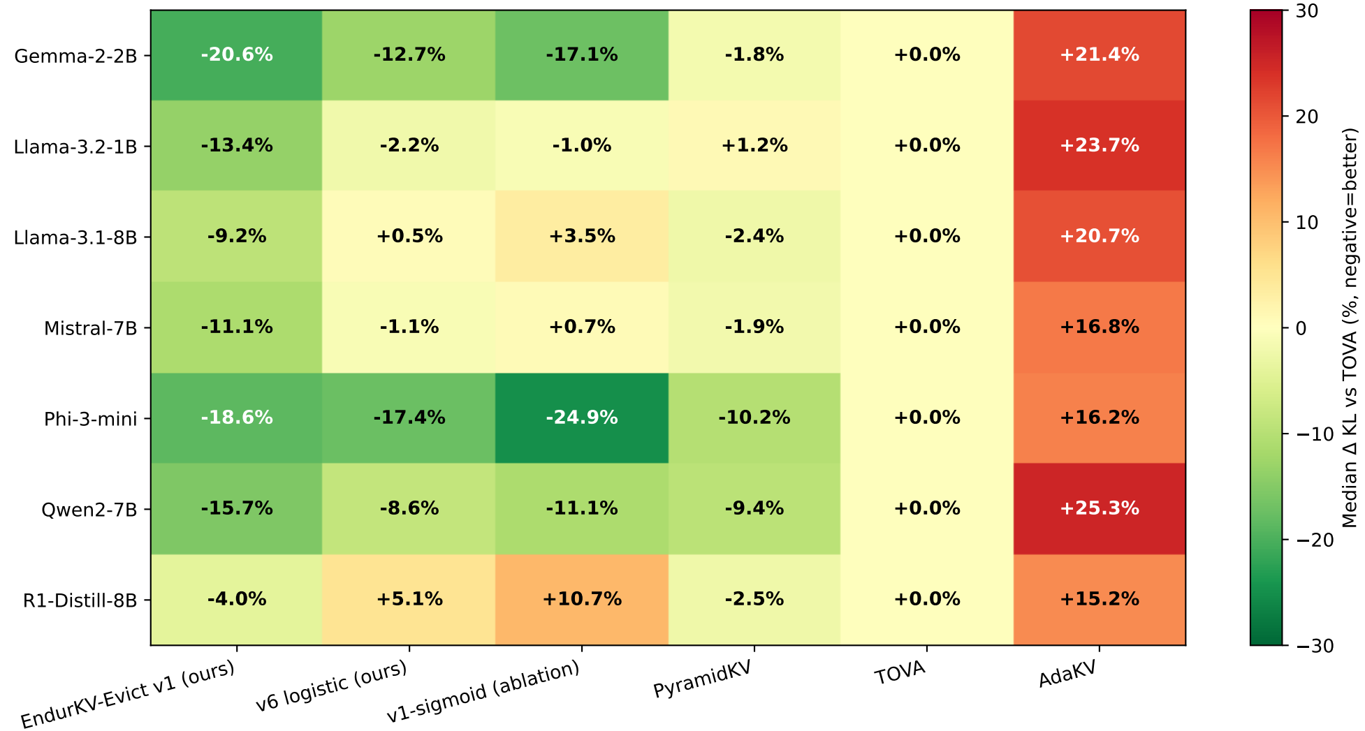
Median \Delta KL vs TOVA — per model \times policy
