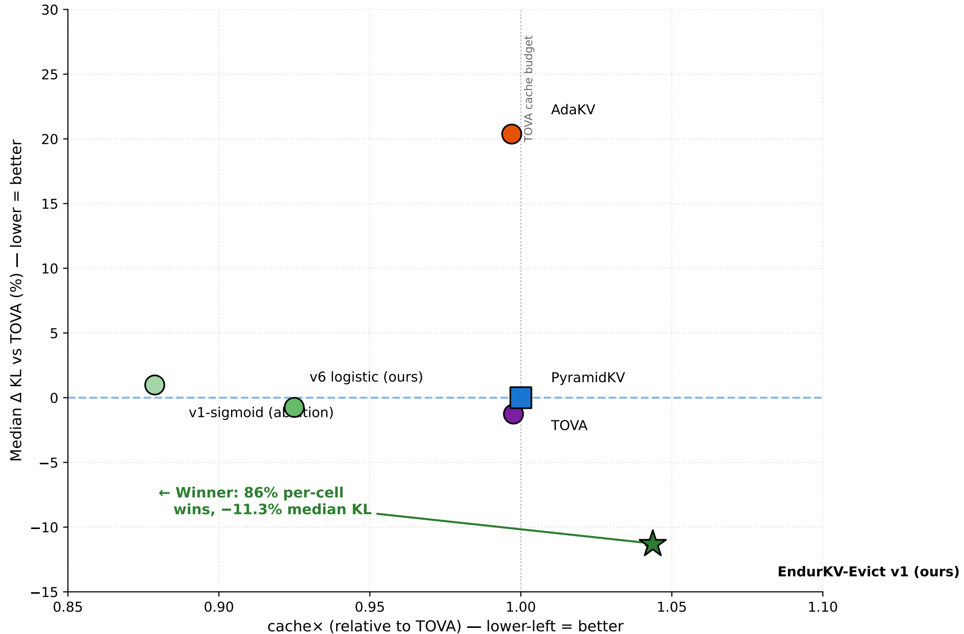
Pareto: cache cost vs quality — 168 cells across 7 models × 5 datasets
