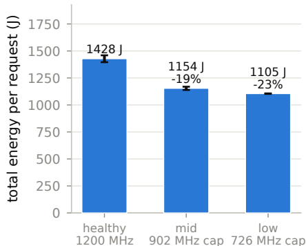
(a) GPU, 4096 output tokens: total energy
