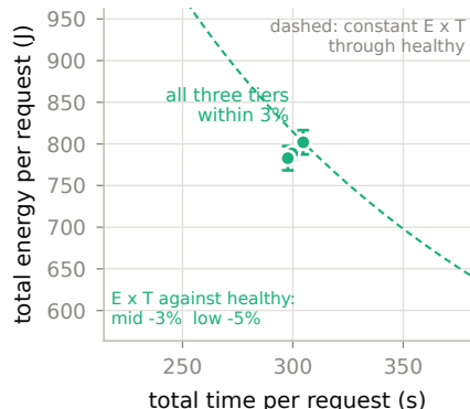
(f) energy against time
