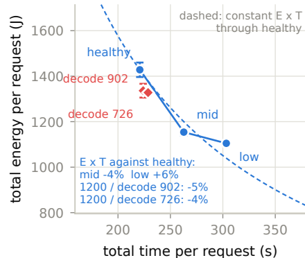
(c) energy against time
