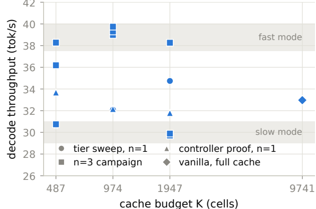
(b) GPU: cache budget vs throughput, every cell
