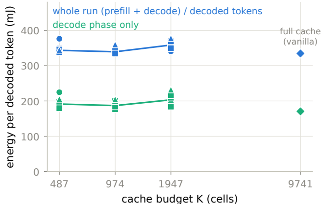
(a) GPU: cache budget vs energy per token
