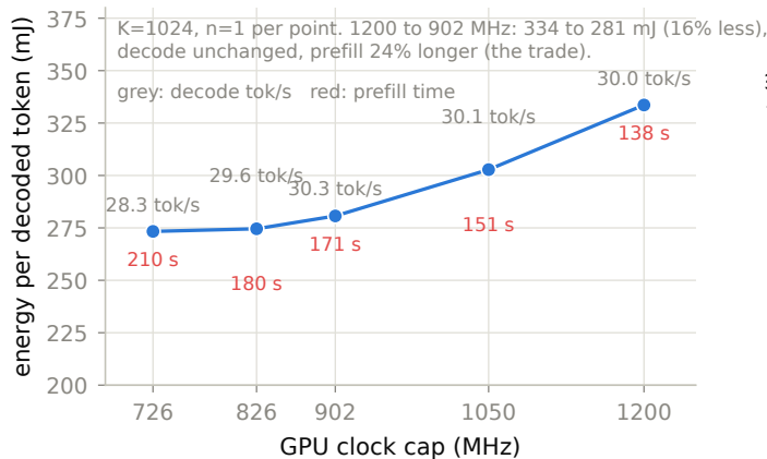
(c) GPU: clock cap vs energy per token
