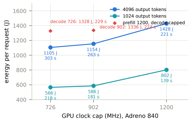
(a) energy against GPU clock cap
