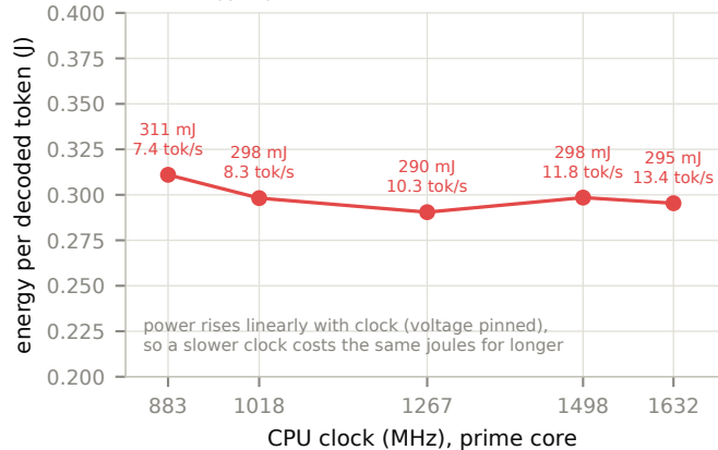
(b) energy against CPU clock: flat within 7%
