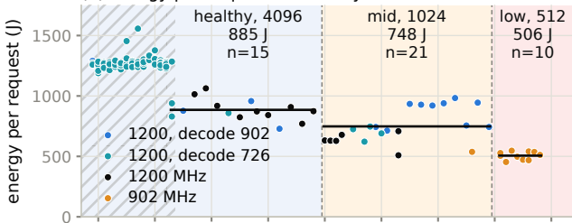
(a) energy per request vs battery level
