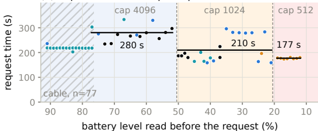
(b) request time and output cap
