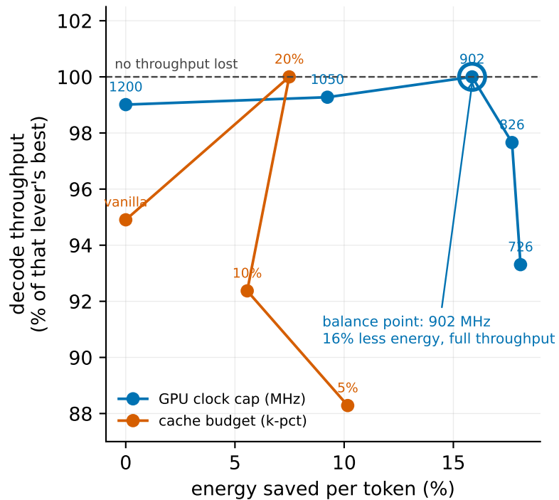
Equilibrium: what each lever costs to save energy
