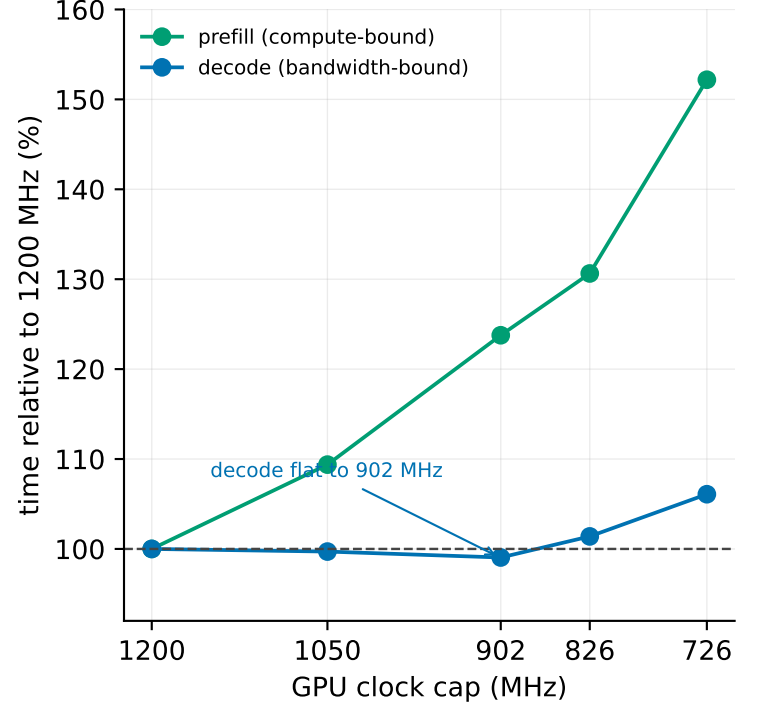
Why: only compute-bound work pays for a lower clock
