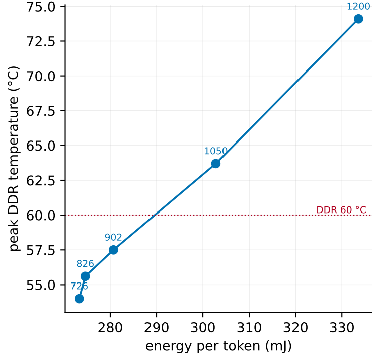
Thermal headroom bought by the clock lever
