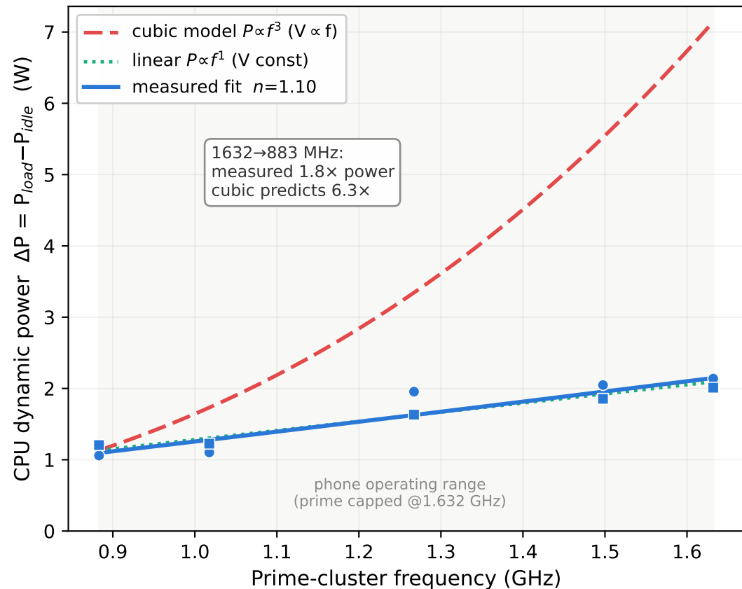
Measured CPU power scales ~linearly with frequency
