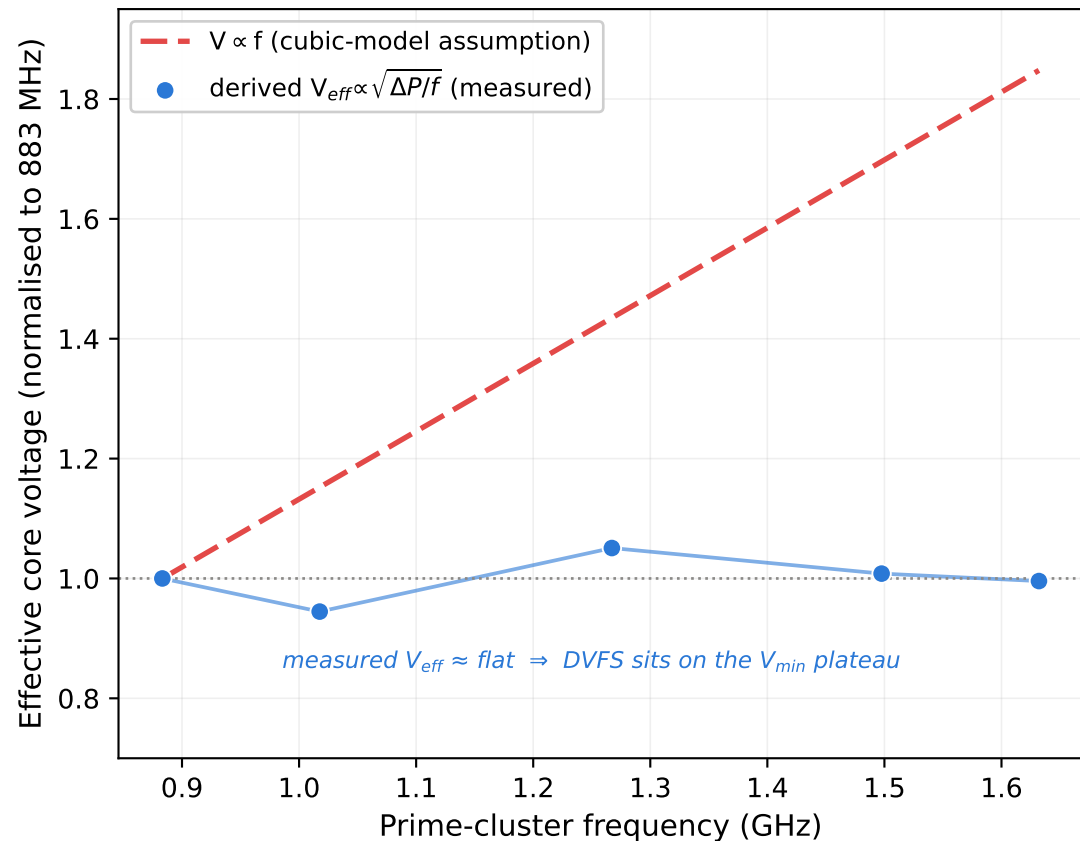
Effective voltage is pinned — no reduction with frequency
