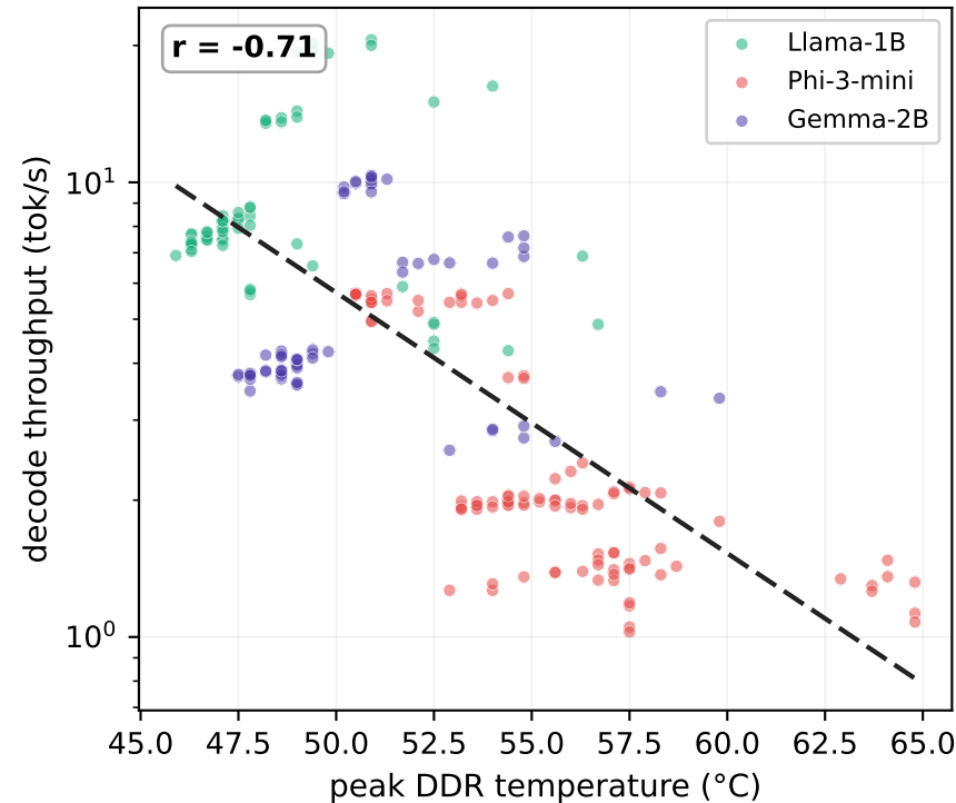
R1 throughput ↔ temperature
