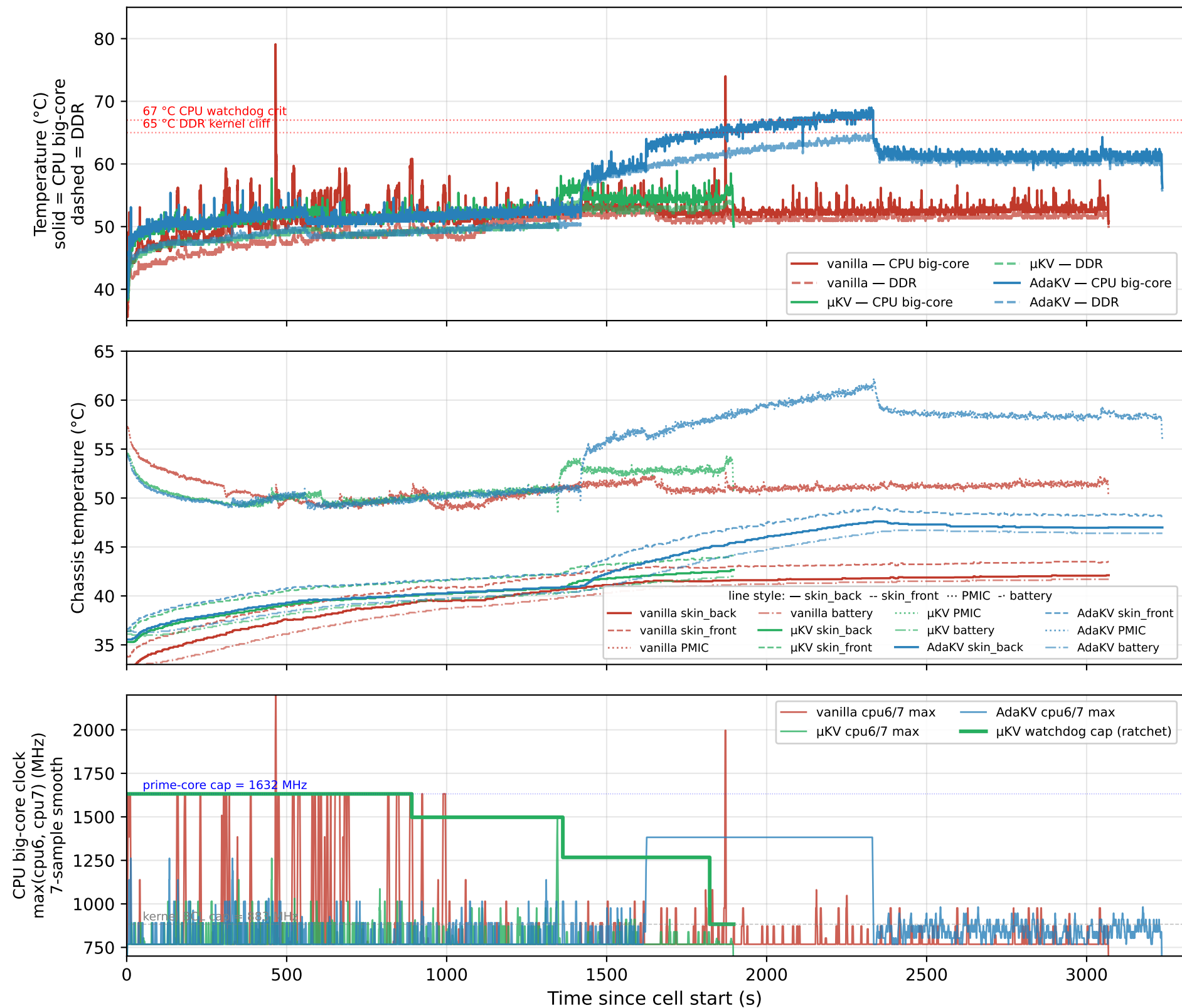
Compute-path thermals (CPU big-core + DDR), chassis thermals, and big-core clock Phi-3-mini, OnePlus 15, 16K decode (14K prompt + 2K decode)
