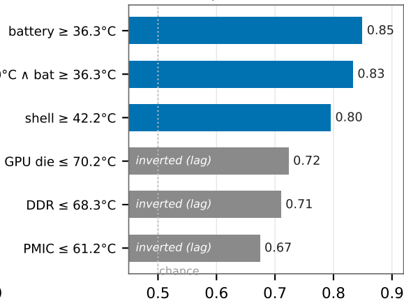
(b) Surface sensors predict the floor; die sensors do not
