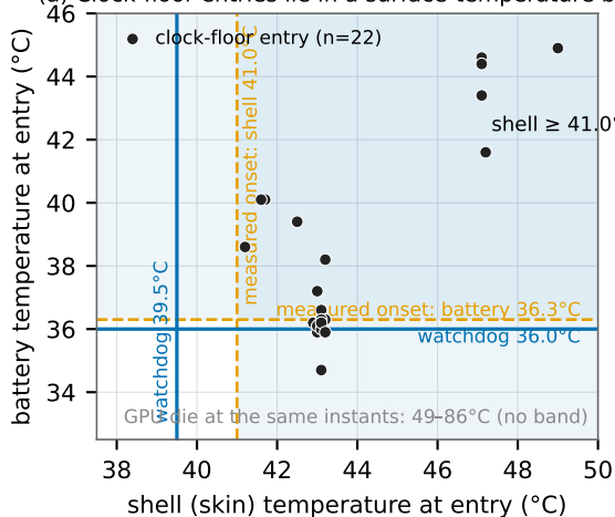
(a) Clock-floor entries lie in a surface-temperature band
