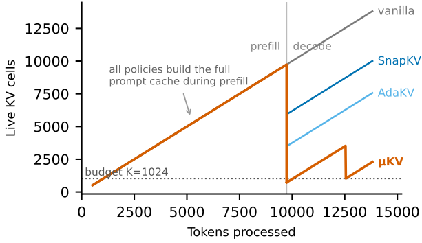
Figure 4: Live KV cells through prefill and decode on Llama-3.2-1B. Only \mu KV compacts to its budget and stays bounded.
