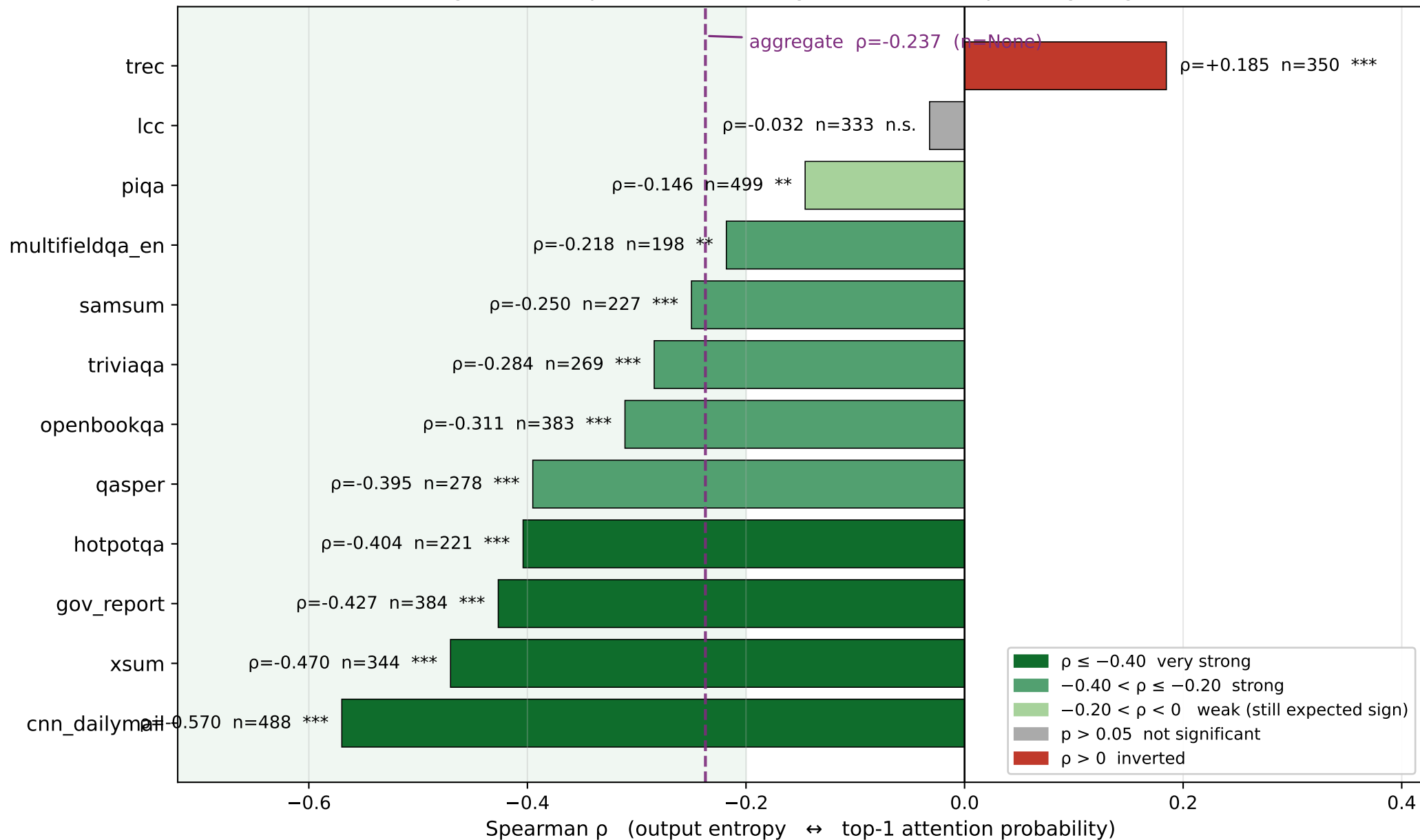
Per-task safety-gate signal across 12 benchmark tasks (green zone: \rho \leq -0.20 = the gate's intended operating range)
