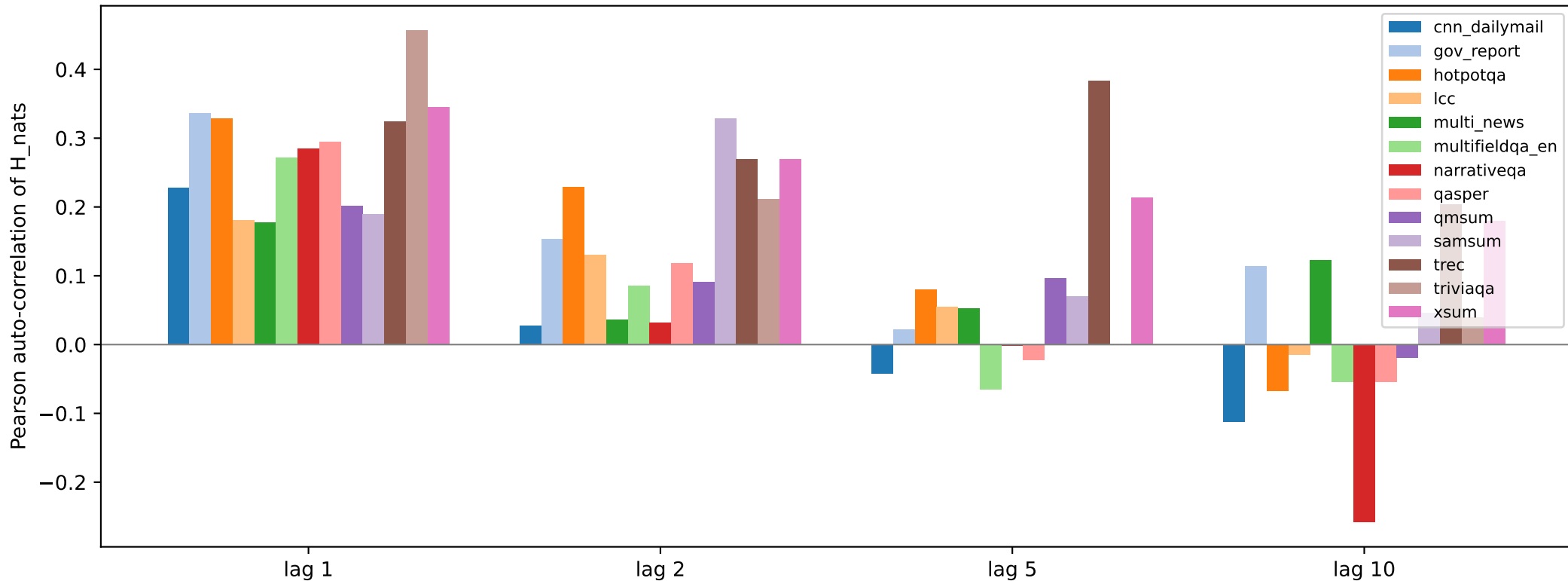
Entropy auto-correlation across decode steps
