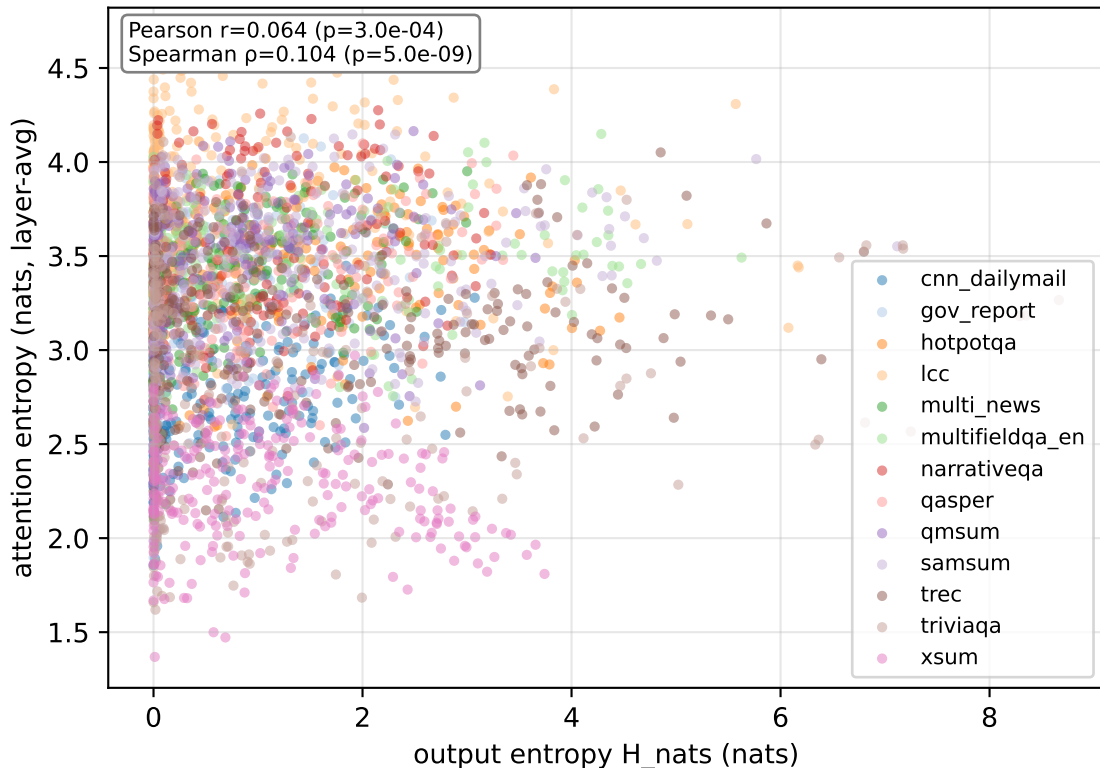
Output entropy vs. attention entropy
