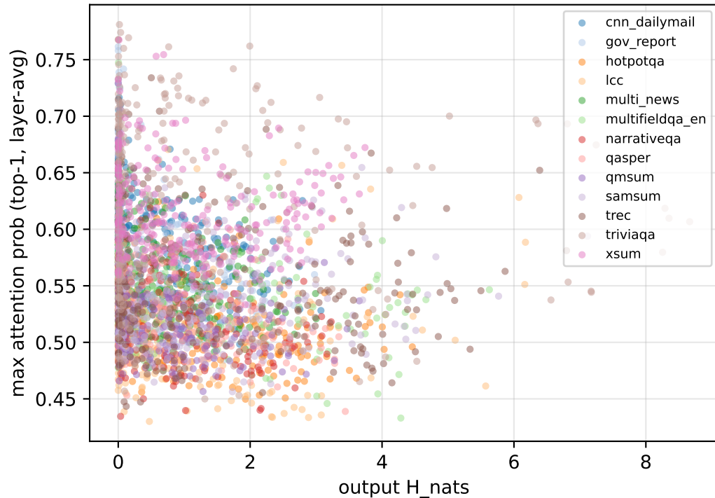
Sharper attention vs. lower entropy \rho=-0.199
