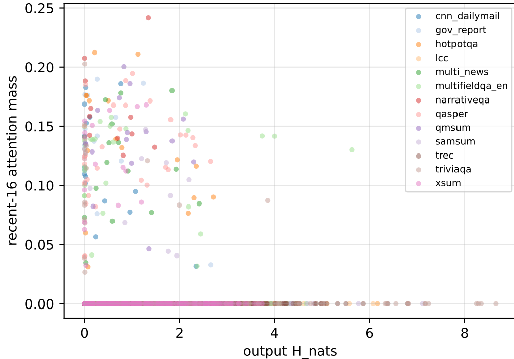
Recent-window mass vs. entropy \rho=-0.038
