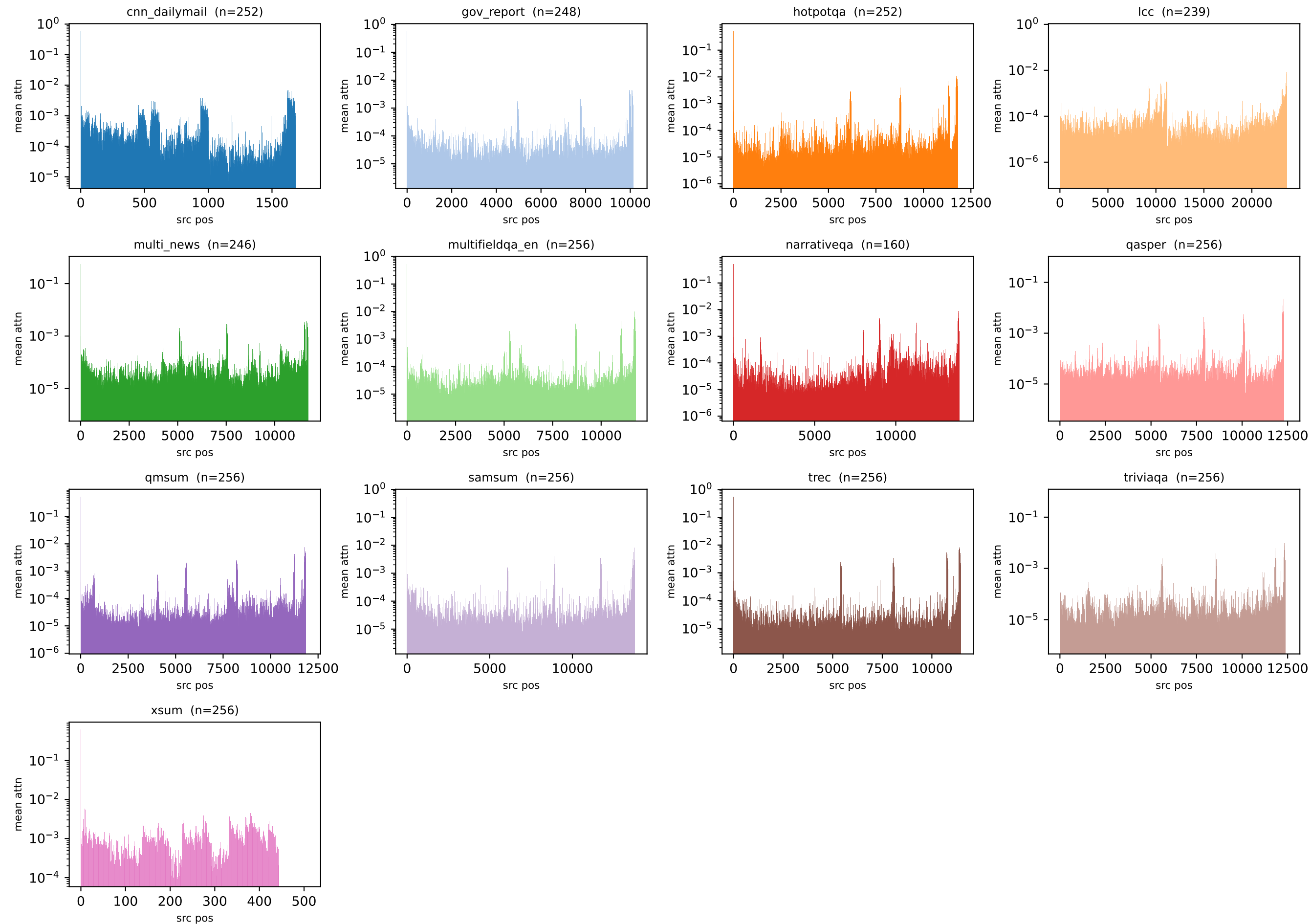
H2O-style heavy-hitter pattern by task (log scale, mean attn prob per source position)
