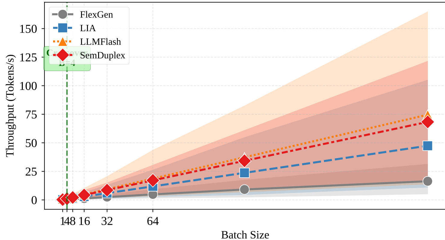
(a) Batch Throughput 72B INT8 16H+32C (tight memory)
