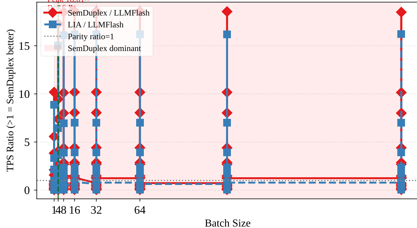
(b) Relative Efficiency vs LLMFlash SemDuplex advantage at B \geq 4
