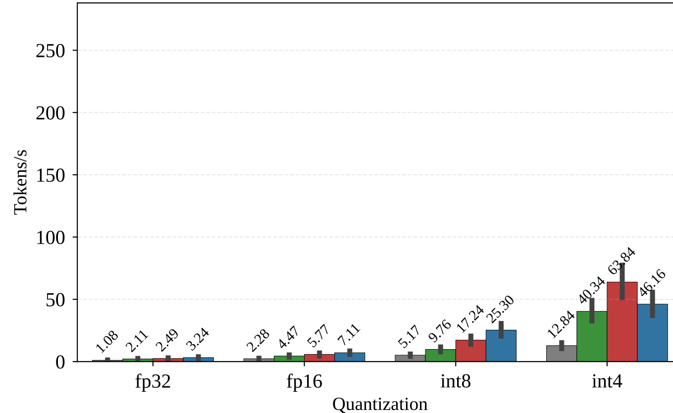
(b) Decode Throughput (16H+32C, B=128)
