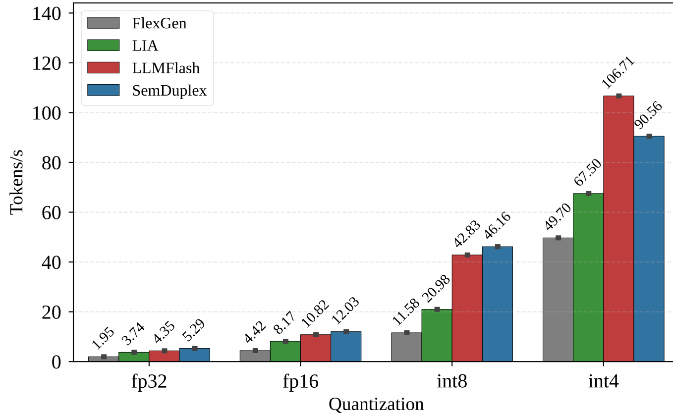
(a) Decode Throughput (32H+32C, B=128)
