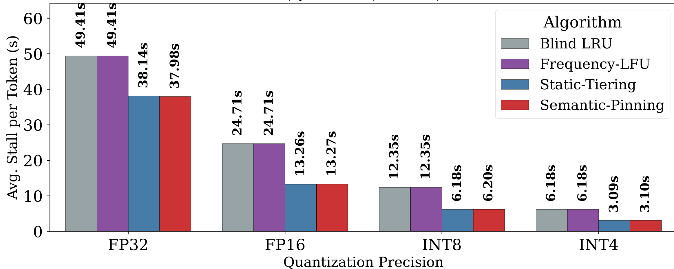
(b) Caching Algorithm Comparison (Qwen 72B, B=128)
