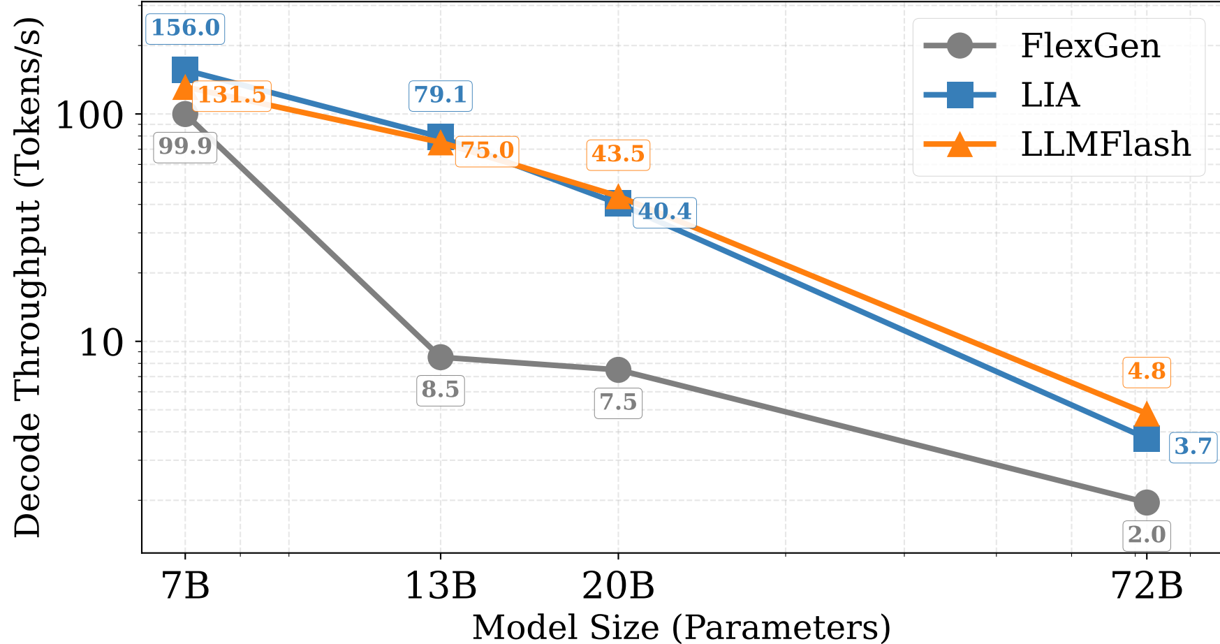
(a) The Latency Wall(Scalability, FP32, B=128)
