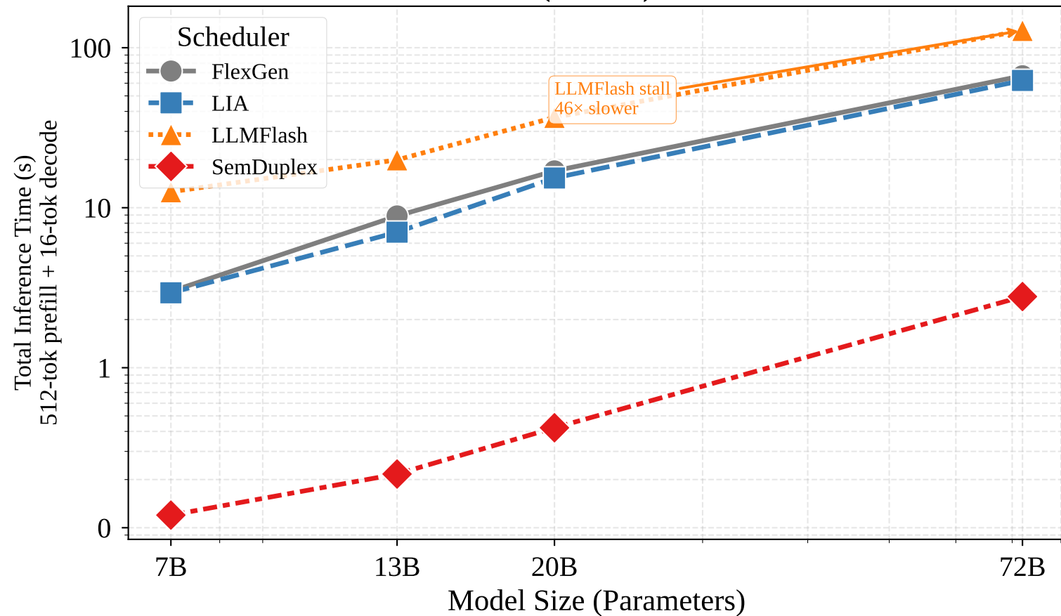
(a) End-to-End Latency Wall (B=128)
