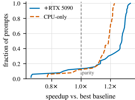
(c) 50 real ShareGPT prompts
