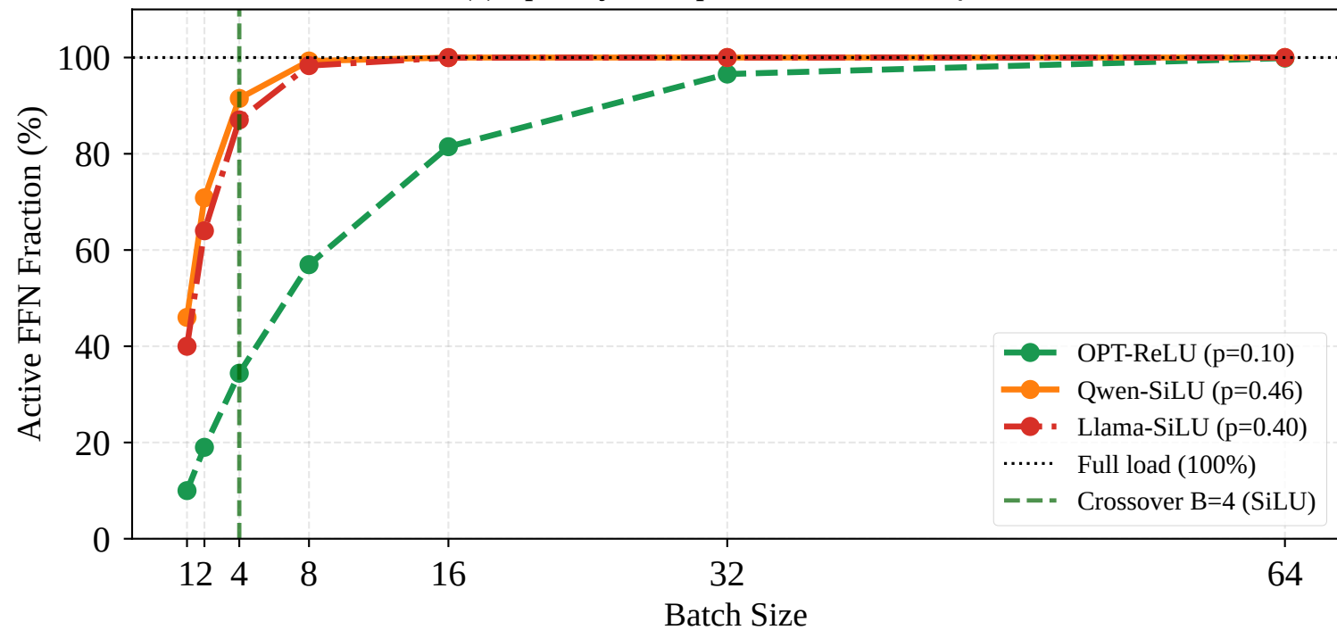
(a) Sparsity Collapse: B \mapsto 1 - (1 - p)^B
