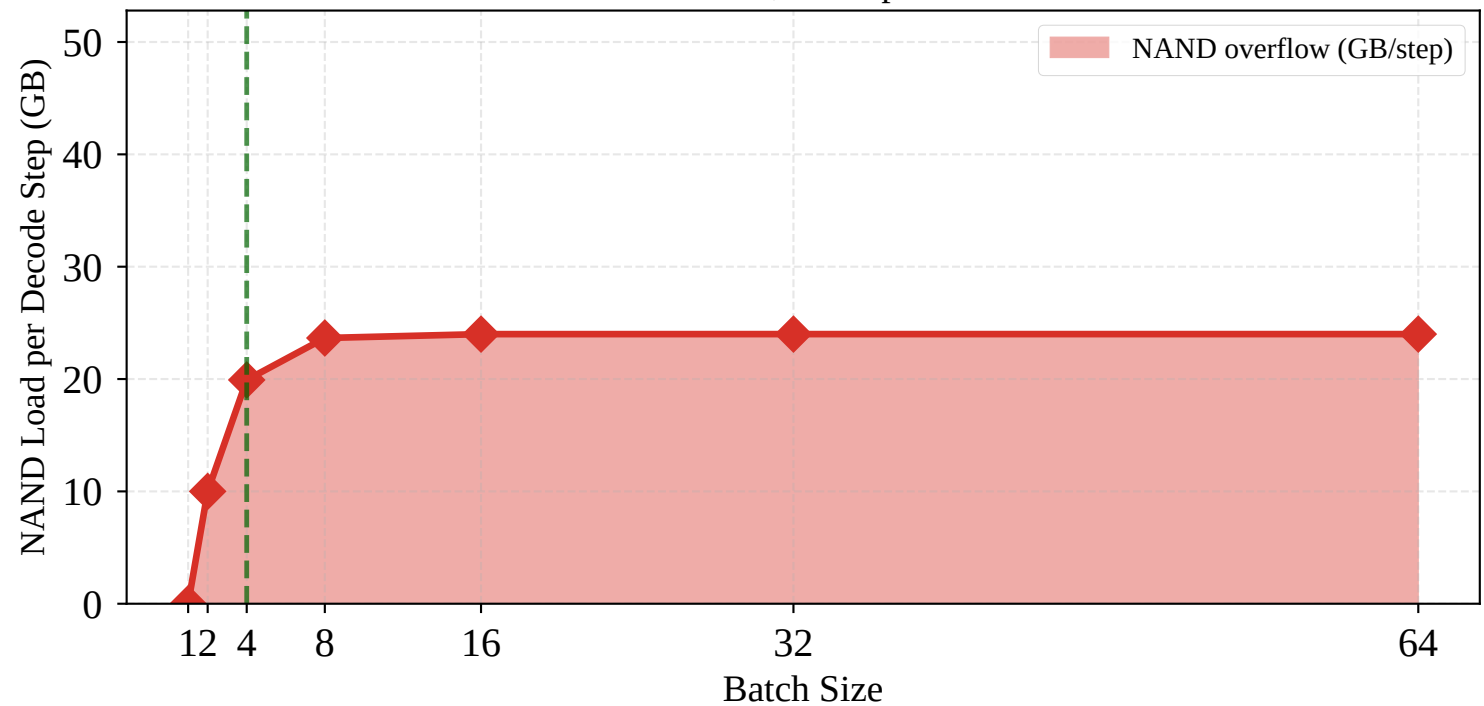
(b) NAND Overflow at 16H+32C 72B INT8, SiLU p=0.46
