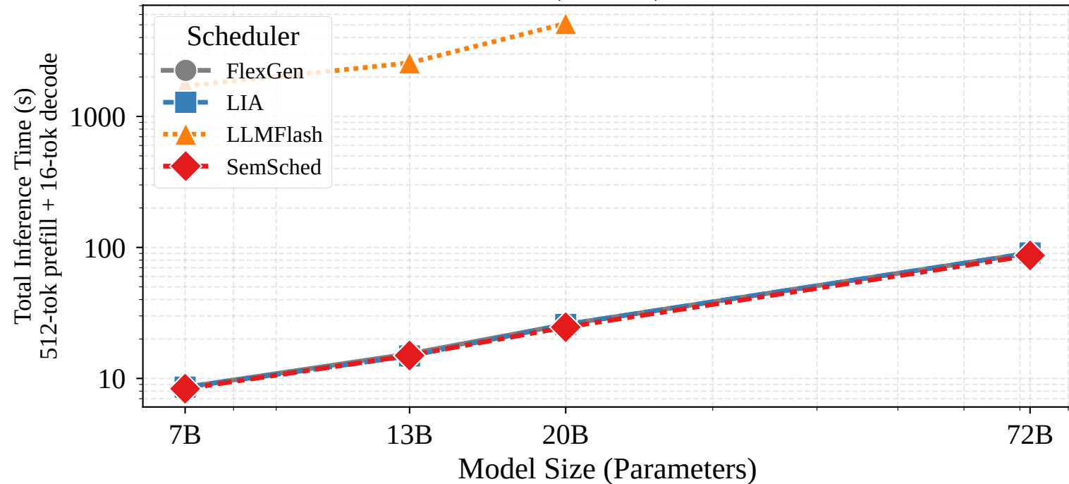
(a) End-to-End Latency Wall (B=128)
