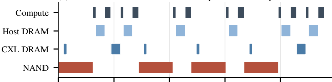
(a) tiers filled: NAND on the critical path — full step 7.12 s
