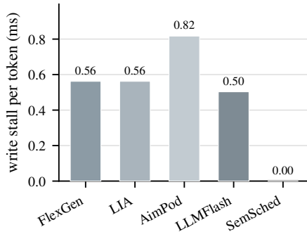
(b) KV write stall, INT8 16H+48C
