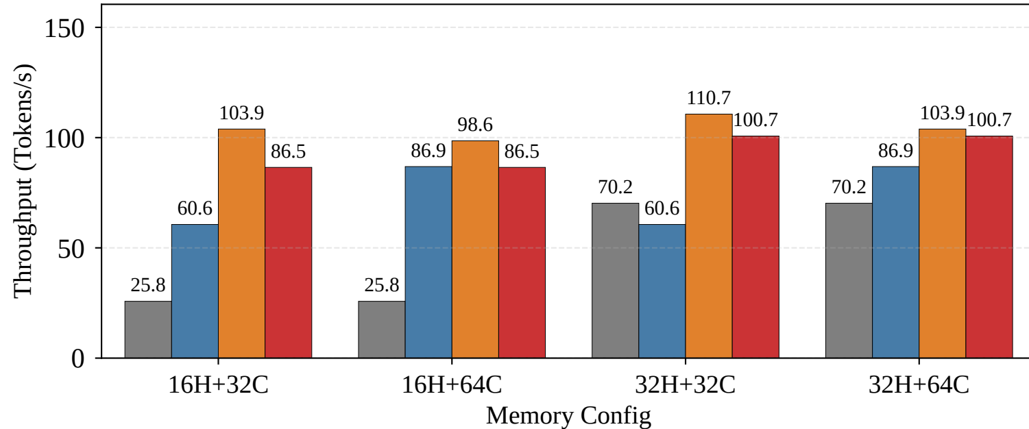
(a) Memory Configuration Sensitivity (72B, INT4, B=128)
