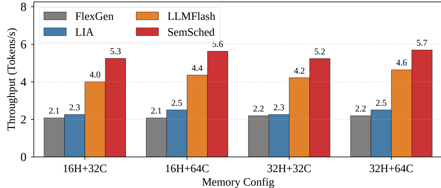
(b) Memory Configuration Sensitivity (72B, FP32, B=128)
