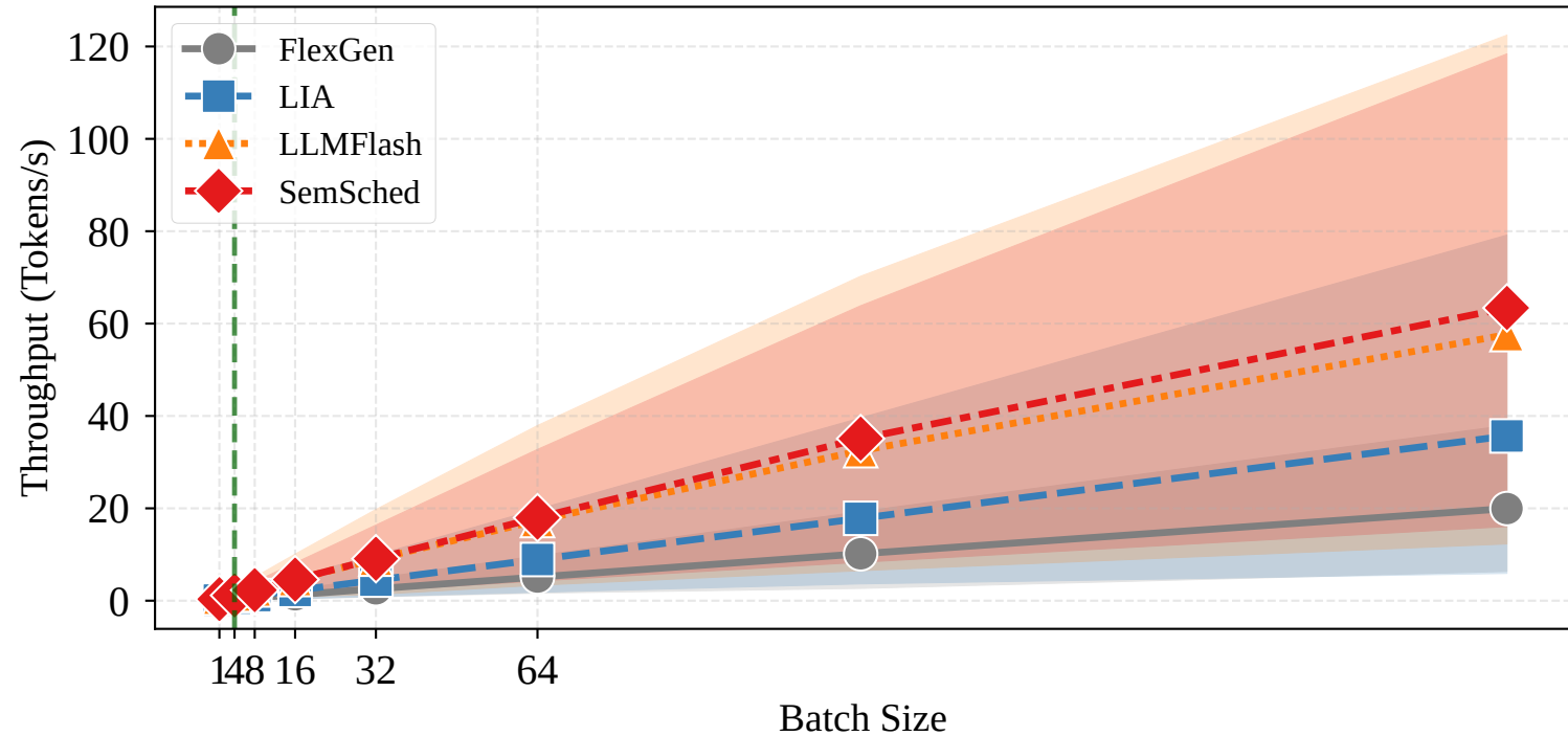
(a) Batch Throughput 72B INT8 16H+32C (tight memory)
