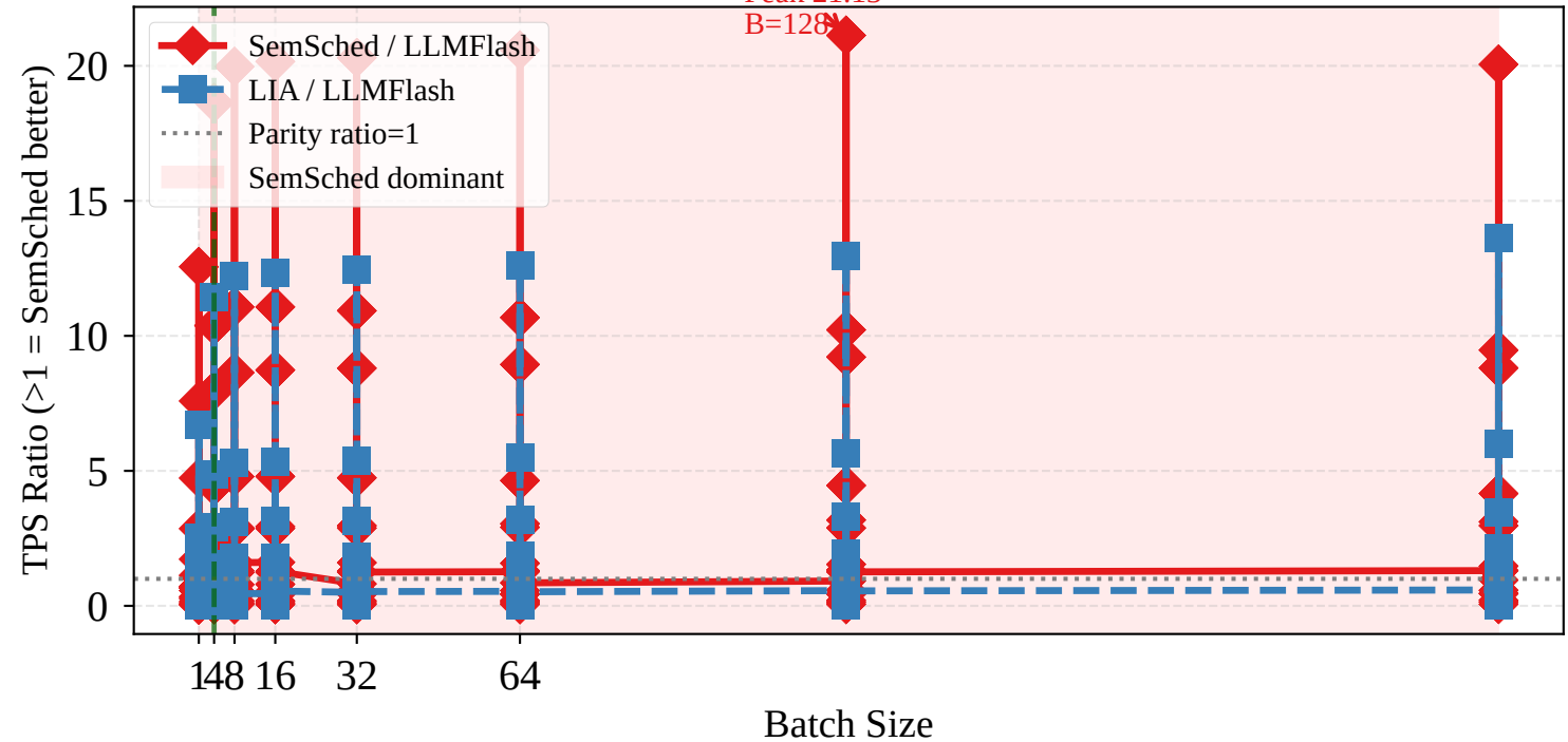
(b) Relative Efficiency vs LLMFlash SemSched advantage at B \geq 4
