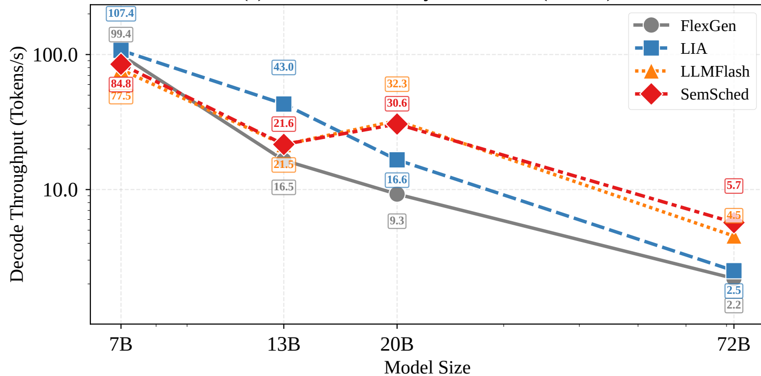
(a) Decode Scalability, 32H+64C, (B=128)
