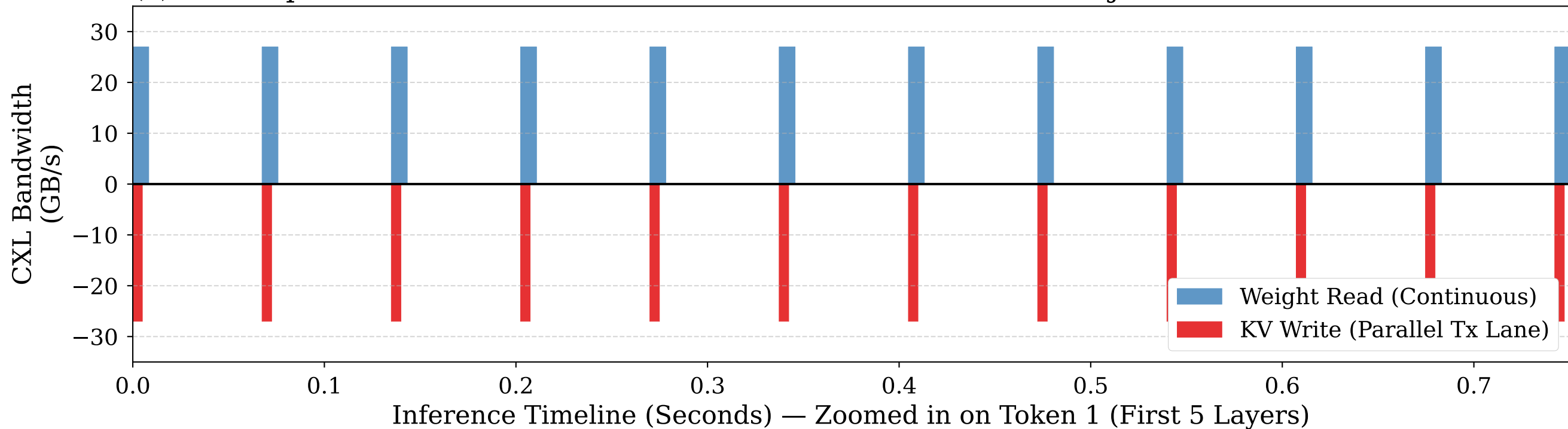
(c) SemDuplex: Continuous Read Stream via Parallel Write Lane Injection
