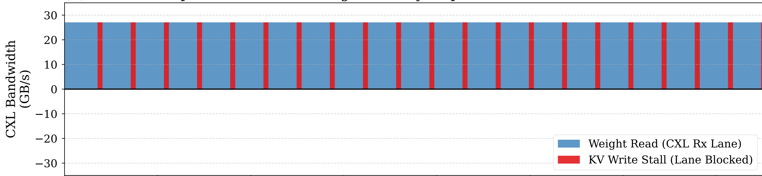
(b) Baseline Simplex: Read Stream Fragmented by Sequential KV-Cache Write Stalls
