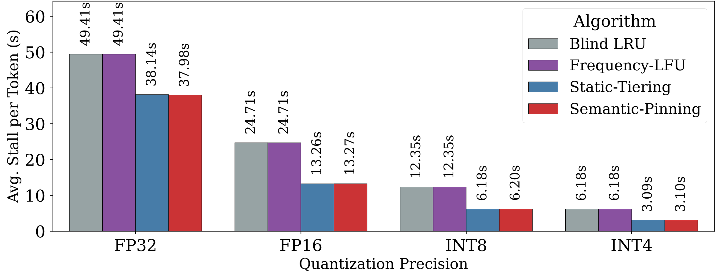
(b) Caching Algorithm Comparison(72B, B=128, 32H+64C)
