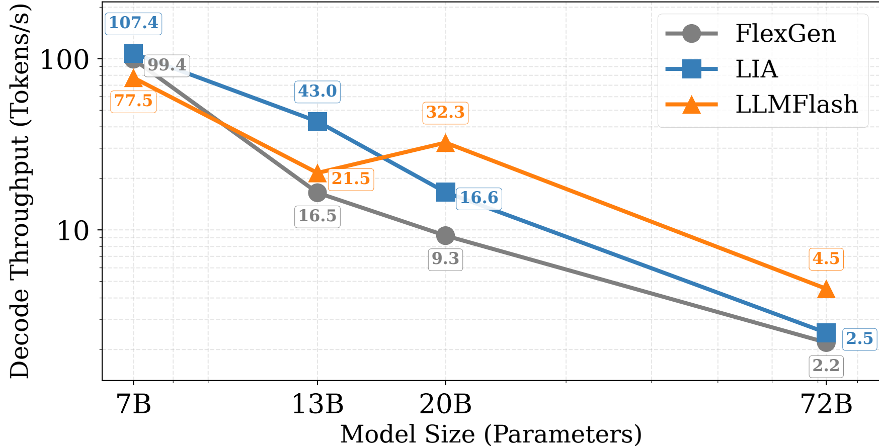
(a) The Latency Wall(Scalability, FP32, B=128, 32H+64C)
