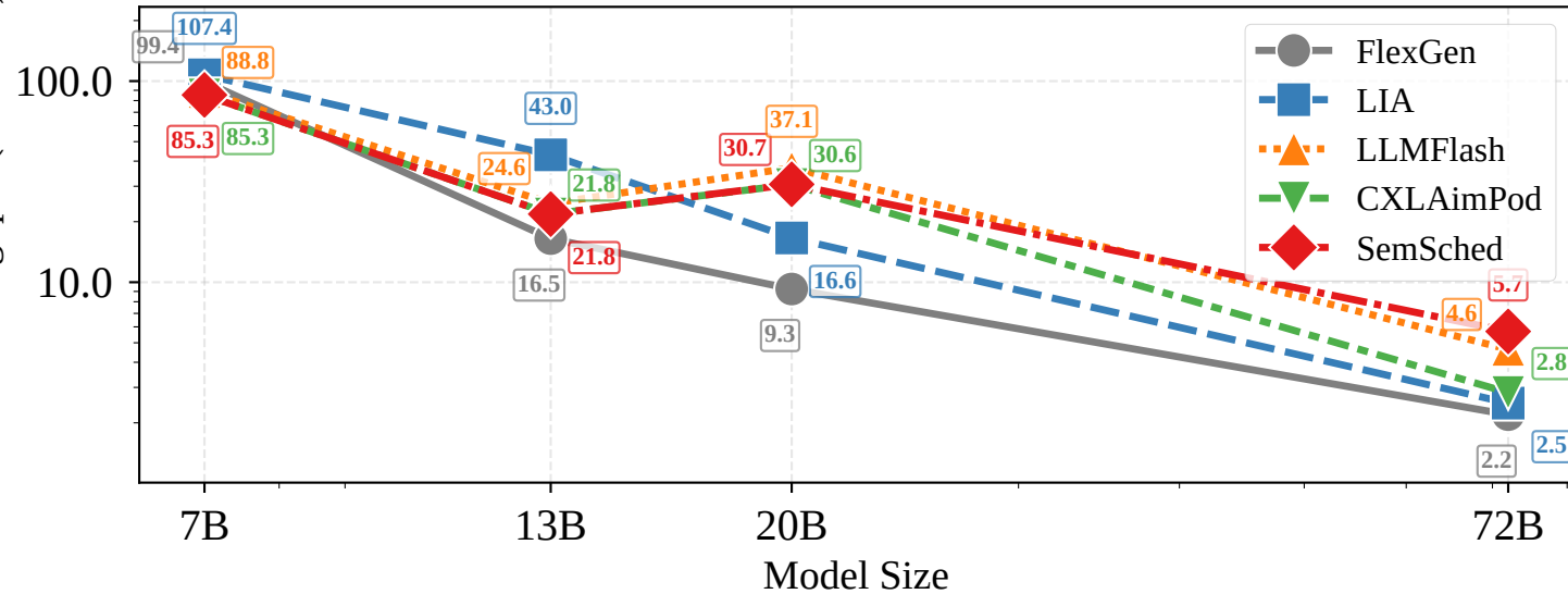
(a) Decode Scalability, 32H+64C, (B=128)
