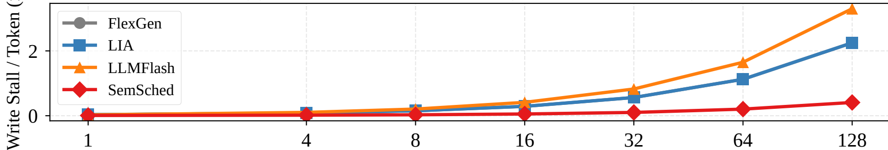
(b) Per-Token Write Stall Time (72B FP32, 16H+32C)
