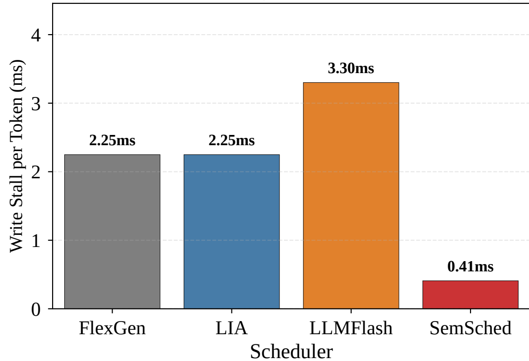
(a) Write Stall / Token (72B FP32, B=128, 16H+32C)
