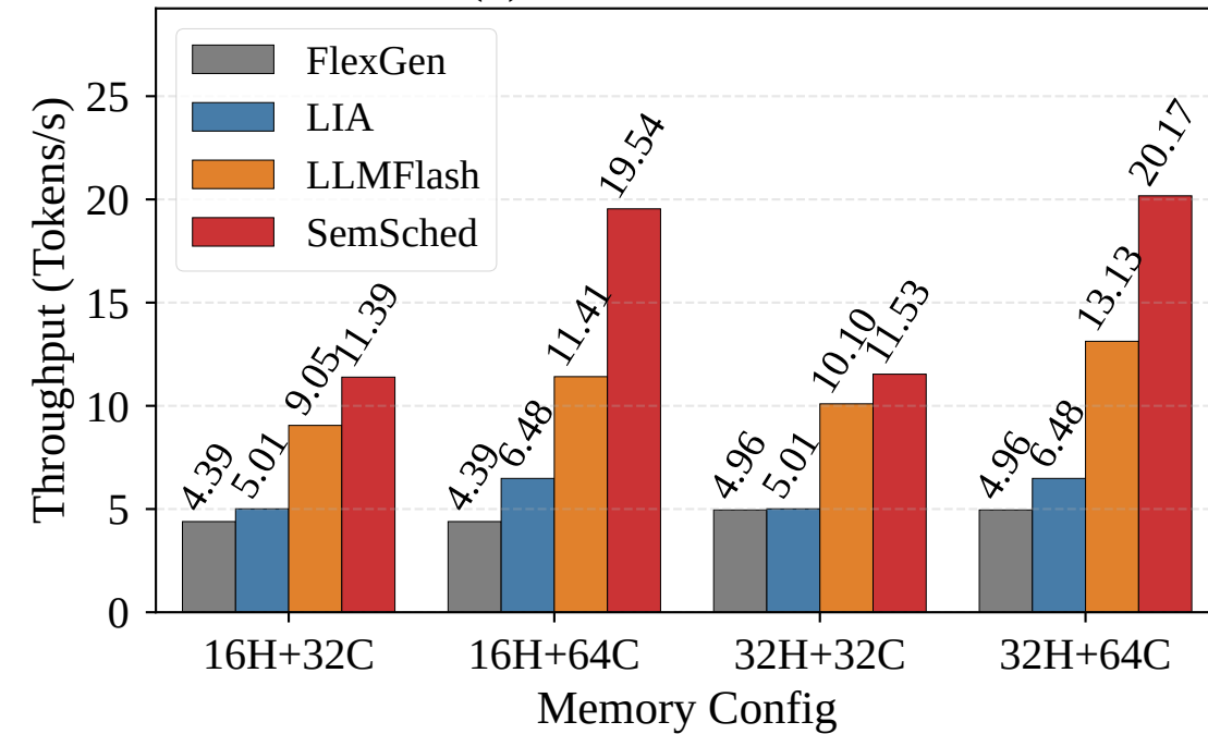
(b) 72B, FP16, B=128
