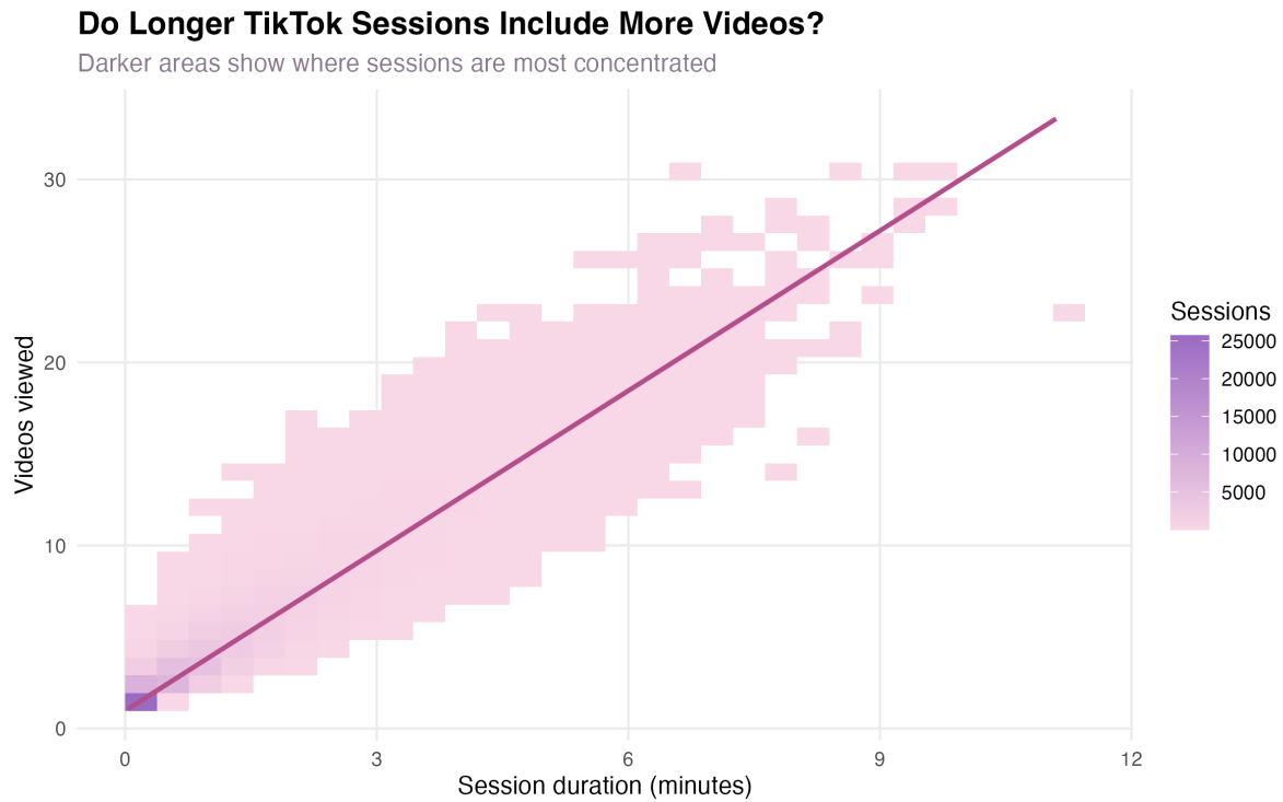
Figure 8: Session duration and videos viewed
