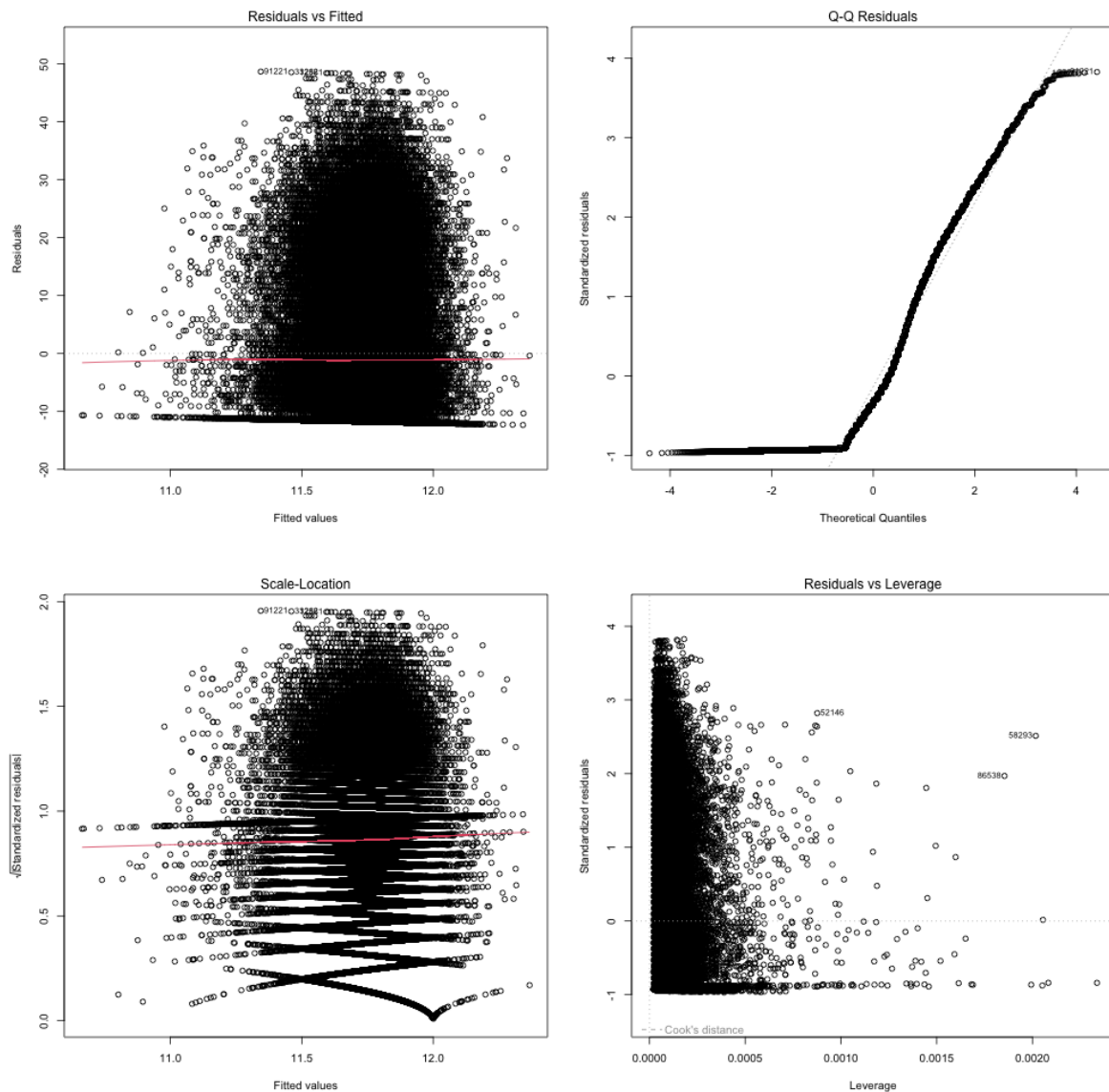
Figure 16: Regression diagnostic plots
