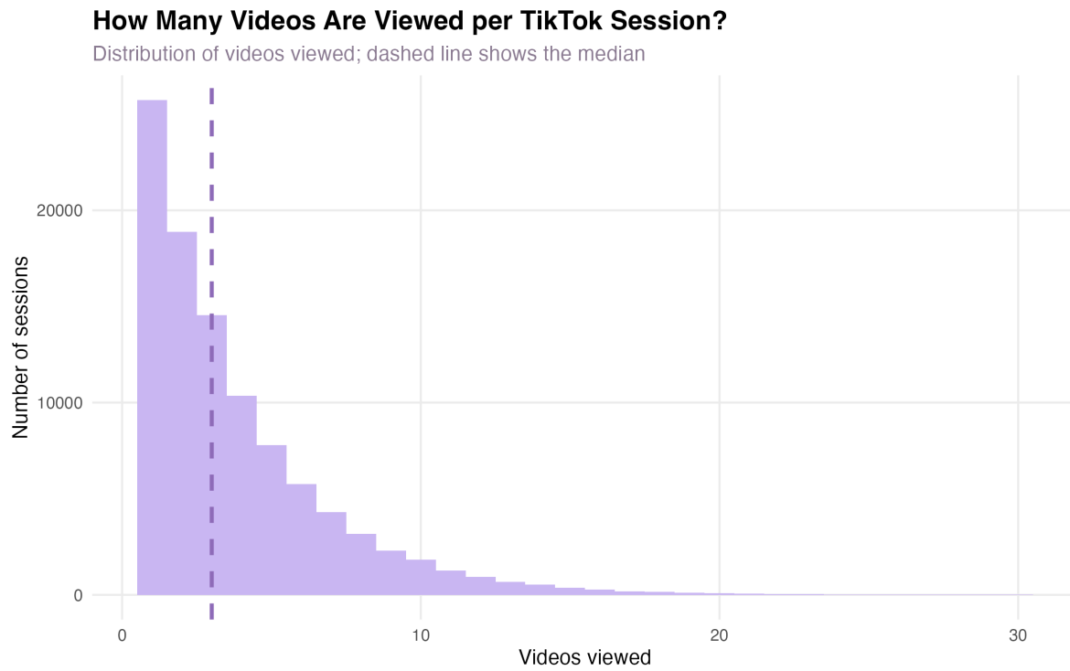
Figure 6: Videos viewed per session
