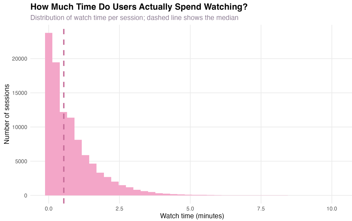
Figure 7: Watch time per session
