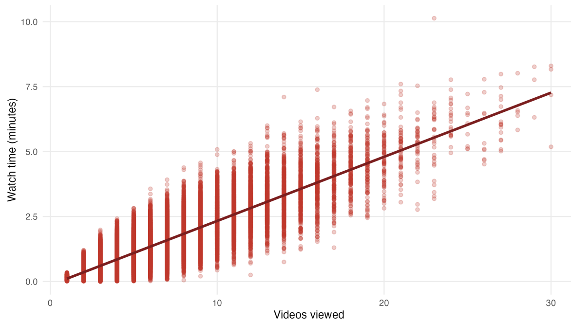
Figure 9: Videos viewed and watch time
