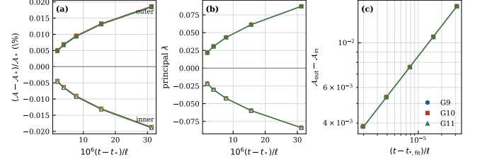
FIG. 1. Three-grid resolution of the free-boundary MOTS saddle-node. (a) One-sided proper cap area relative to the gridwise near-critical reference area A_* at the selected bracket endpoint, not an exact critical value; filled symbols denote the outer branch and open symbols the inner branch. (b) The corresponding principal stability eigenvalues, which approach zero with opposite signs. (c) Log-log area separation and the gridwise fits \Delta A = [s(t - t_*, \text{fit})]^{1/2} .
