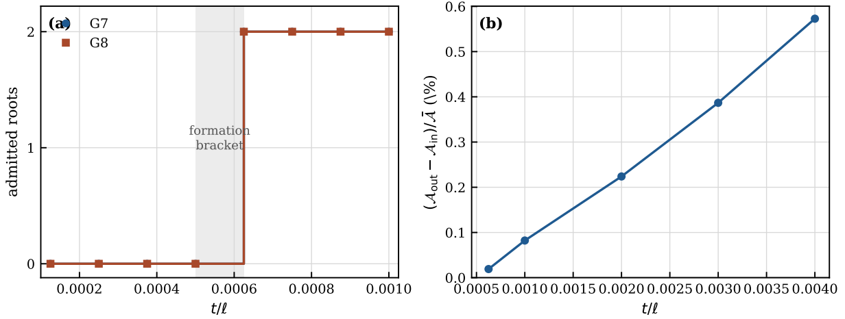
Figure 1: Historical pre-repair realization, retained for provenance and not used as independent support for the repaired result. Left: admitted upper-brane-capped root count on the two G7/G8 grids. Both histories change from zero to two in the common formation bracket. Right: one-sided proper cap-area separation on G8, shown relative to the mean area at each sampled time. The earliest positive gap is not claimed as quantitatively resolved; the growing separation on later slices is.
