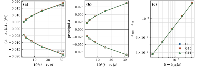
FIG. 1. Three-grid resolution of the free-boundary MOTS saddle-node. (a) One-sided proper cap area relative to the gridwise near-critical reference area \mathcal{A}_* at the selected bracket endpoint, not an exact critical value; filled symbols denote the outer branch and open symbols the inner branch. (b) The corresponding principal stability eigenvalues, which approach zero with opposite signs. (c) Log-log area separation and the gridwise fits \Delta\mathcal{A} = [s(t - t_*, \text{fit})]^{1/2} .
