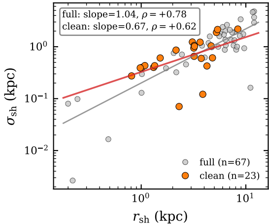
Width-radius scaling
