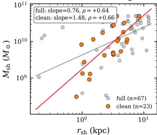
Mass-radius scaling
