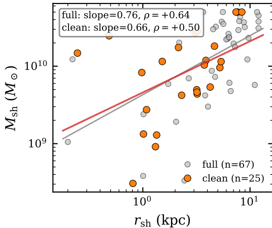
Mass-radius scaling
