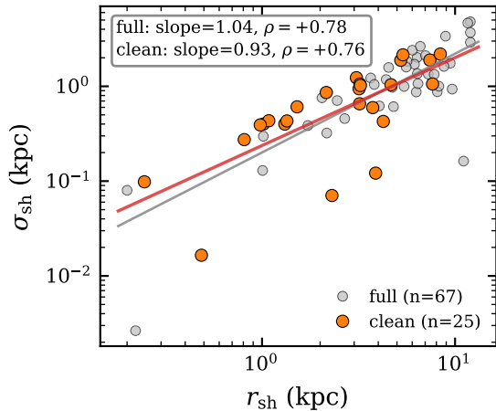
Width-radius scaling
