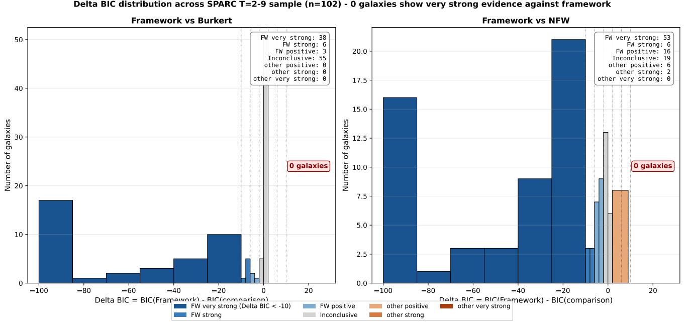
Figure 1. \Delta\text{BIC} distribution across the SPARC T=2–9 sample ( n=102 ). The histograms make visible the asymmetry: zero galaxies fall in the very strong evidence against framework region ( \Delta\text{BIC} > +10 ) for either comparison.
