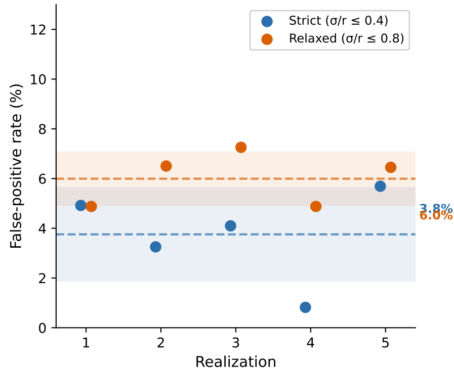
(a) Null-curve FP rate per realization
