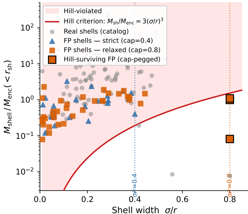
(b) Hill criterion: FP shells vs real shells
