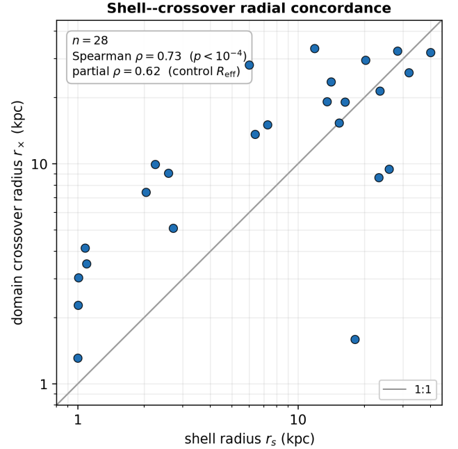
Figure 2. Radial concordance between the two decompositions. For the n = 28 galaxies hosting both a BIC-selected second domain and an independently fitted shell, the domain crossover radius r_x is plotted against the nearest shell radius r_s (logarithmic axes); the solid line is r_x = r_s . The two radii are strongly correlated (Spearman \rho = 0.73 ), and the correlation survives control for the optical half-light radius (partial \rho = 0.62 ), so the two methods localize structure to common radii for reasons beyond a shared preference for the mid-disk.
